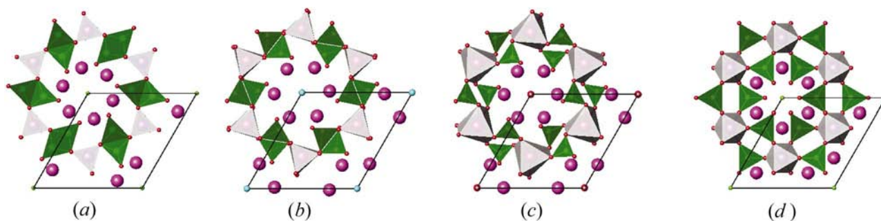
Figure 8 The preferred topological representation of four apatites; both the A(1)O_6 trigonal prisms/metaprisms and the BO_4 tetrahedra are emphasized. The idealized structural endmembers are emphasized in (a) model I with \varphi = 0^\circ and (d) model III with \varphi = 60^\circ . The intermediate structures shown are for (b) hedyphane Ca 4 Pb 6 (AsO 4 ) 6 Cl 2 with \varphi = 5.2^\circ and (c) Pb 10 (PO 4 ) 6 (OH) 2 with \varphi = 26.7^\circ .
