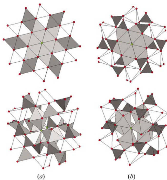
Figure 7 Arrangement of cation-centred polyhedra in (a) model II, which approximates the arrangement in fluorapatite, and (b) the refined structure of fluorapatite. In the upper part the projection along [001] is shown, while A(1)O_6 , A(2)O_5X and BO_4 connectivity is emphasized in the lower clinographic projections.
